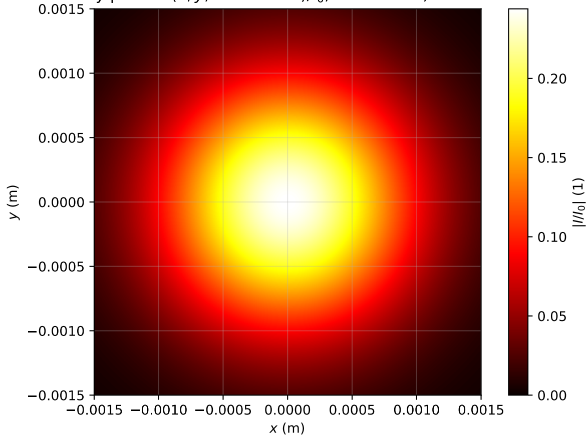
Intensity profile I(x, y, z = 3.742m)/I_0 , P_{in}=0.1P_{cr} , artificial time
